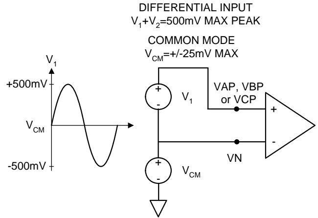
Figure 12. Maximum input level, voltage channels, Gain=1
