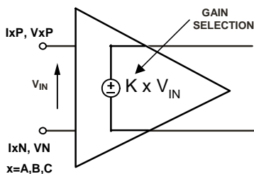
Figure 11. PGA in current and voltage channels
