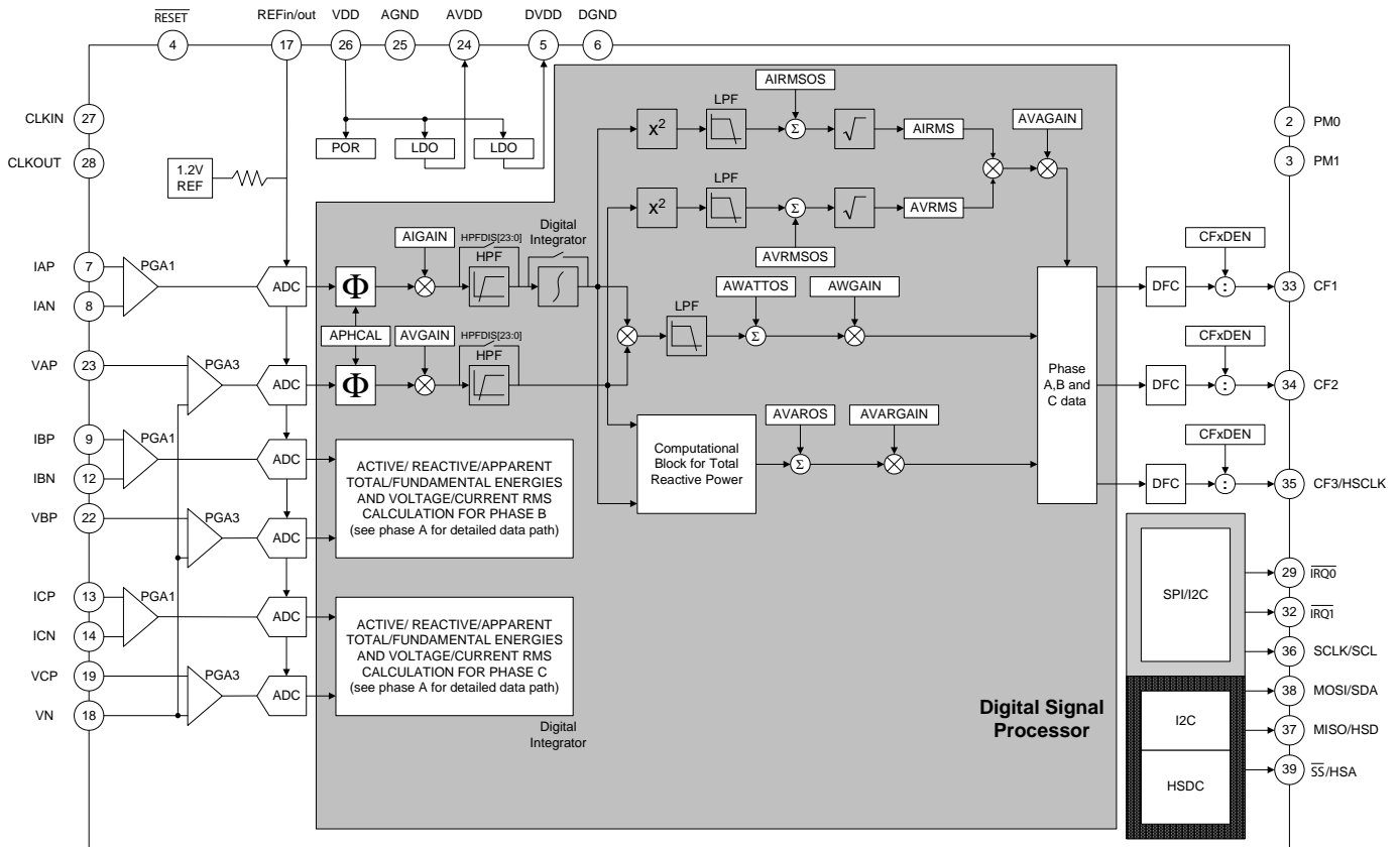
Figure 1. ADE7854 Functional Block Diagram
